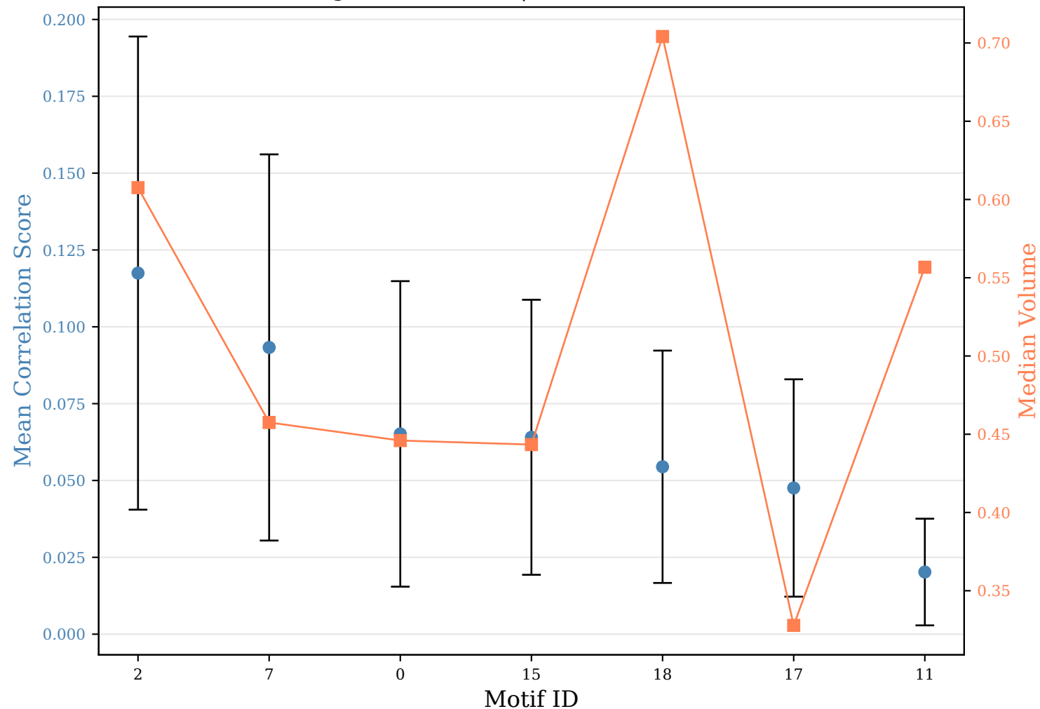
Mean Correlation Score & Median Volume per Motif (Downsampled, sorted by score) sigma: (0.02, 0.4) | volume: (0.03, 0.9)
